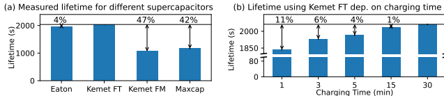
Figure 1: Lifetime of an MSP430-based sensor node powered by different supercapacitors (a) and by a single supercapacitor charged for different amounts of time (b).
