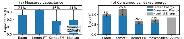
Figure 2: Measured capacitance (a) and energy leakage (b) of different supercapacitors.
