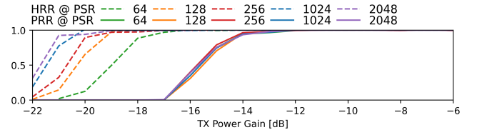
Fig. 6: Impact of PSR on the reliability of communications. Higher PSR values increase the reliability of the HRR, whereas the PRR is unaffected. A PAC size of 16 was used in these experiments.
