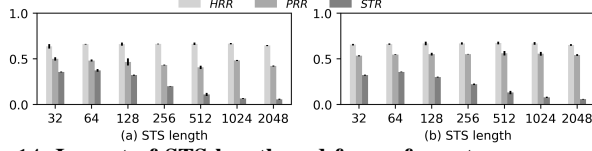
Fig. 14: Impact of STS length and frame format on communication under Wi-Fi 6E interference in HALLWAY. Short STS lengths increase the STR; the use of the SP2 frame format increases the PRR.
