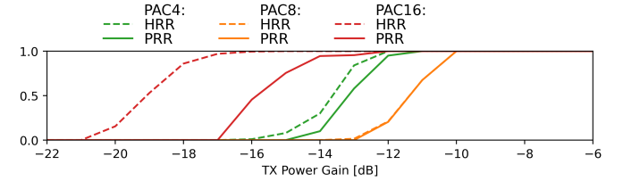
Fig. 8: Impact of PAC size on the reliability of communications. A PAC size of 16 leads to the highest HRR and PRR, whereas a PAC size of 8 results in the lowest receiver sensitivity.
